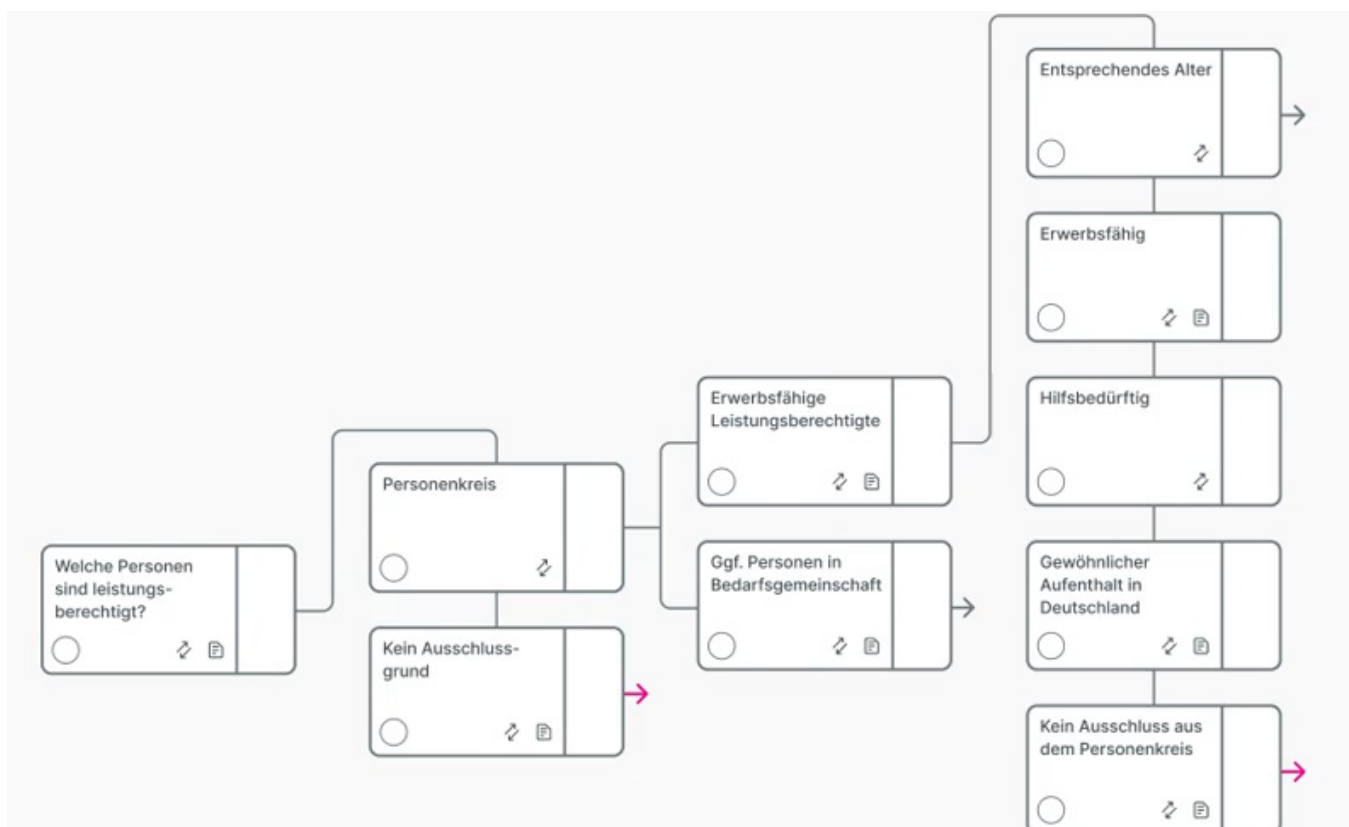
Abb. 05-1: Rule Mapping
