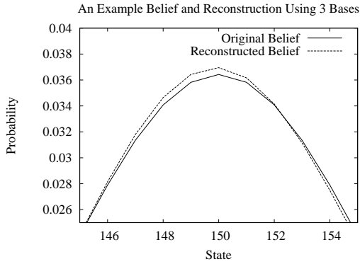
(c) Example Belief and Reconstruction Near Peak
