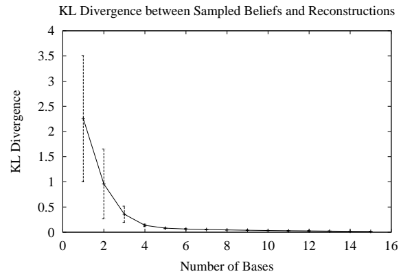
(b) Reconstruction Performance
