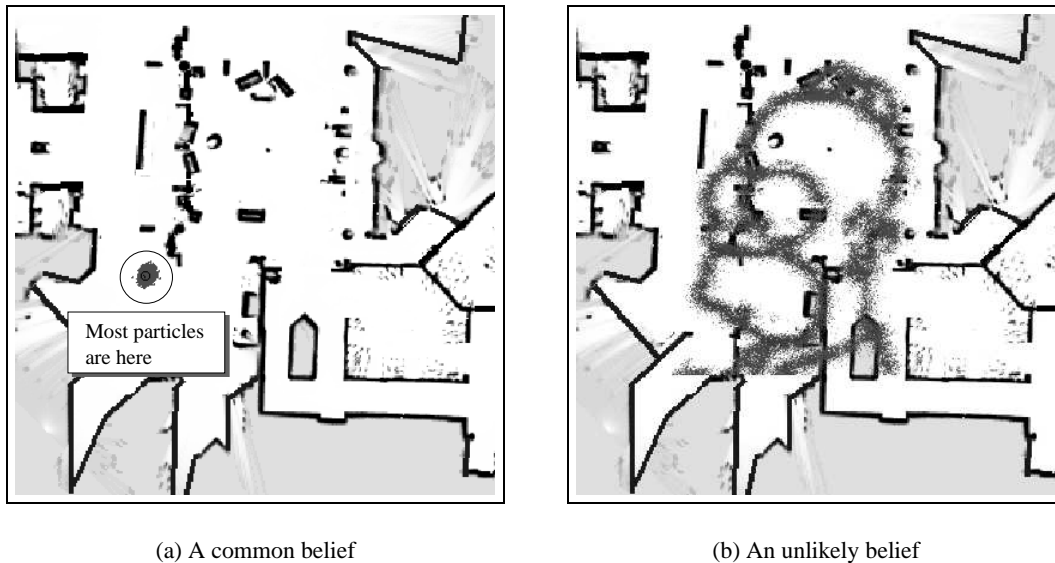
Figure 4: Two example probability distributions over robot pose. The small black dots are particles drawn from the distribution over discrete grid positions. On the left is a distribution where the robot’s location is relatively certain; this kind of compact, unimodal distribution is very common in robot navigation. On the right is a very different, implausible distribution. The right hand distribution is sufficiently unlikely that we can afford to ignore it; even if we are unable to distinguish this belief from some other belief and as a result fail to identify its optimal action, the quality of our controller will be unaffected.
