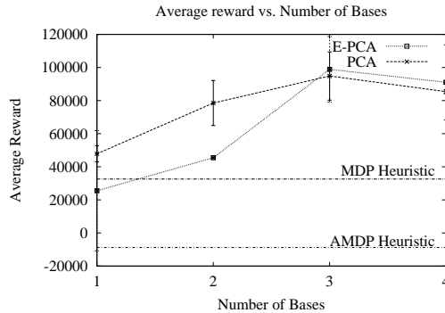
Figure 15: A comparison of policy performance using different numbers of bases, for 10000 trials, with regular grid discretization. Policy performance was given by total reward accumulated over trials.
