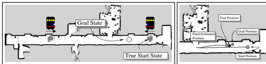
Figure 16: An example robot trajectory, using the policy learned using 5 basis functions. On the left are the start conditions and the goal. On the right is the robot trajectory. Notice that the robot drives past the goal to the lab door to localize itself, before returning to the goal.
